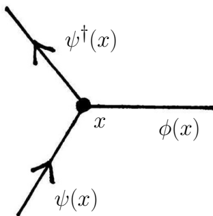
Fig. 20.1 The \psi^\dagger\psi\phi interaction vertex.
