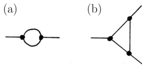
Fig. 32.5 Two divergent diagrams occurring in \phi^3 theory.
