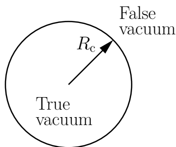
Fig. 50.15 The bubble in Euclidean space.
