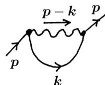
Fig. 43.3 The Fock contribution to the self-energy \Sigma_{\mathbf{p}}^{(F)} .
