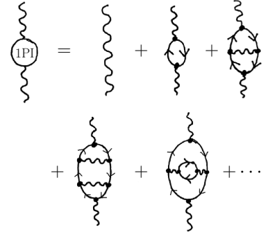
Fig. 41.2 Some contributions to the Green’s function i\tilde{\Pi}^{\mu\nu}(q) .
