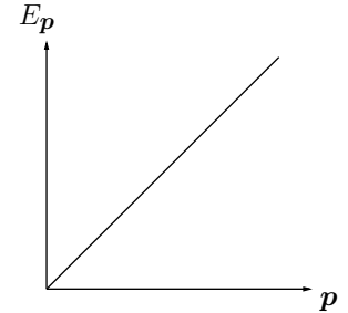
Fig. 7.1 The dispersion relation E_{\mathbf{p}} = |\mathbf{p}| .
