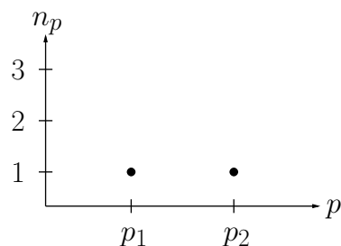
Fig. 3.1 A two-particle state given by |p_1p_2\rangle .
