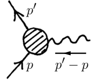
Fig. 41.7 The vertex Green's function -iQ|e|\Gamma^\mu(p, p') .
