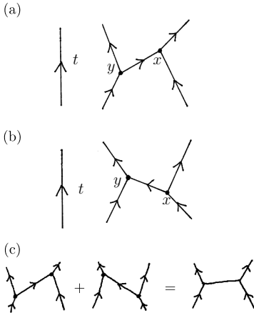
Fig. 17.4 (a) A virtual particle propagates from y to x mediating a force. (b) The same process occurs with a virtual particle propagating from x to y . (c) The processes are summed to make the Feynman propagator.
