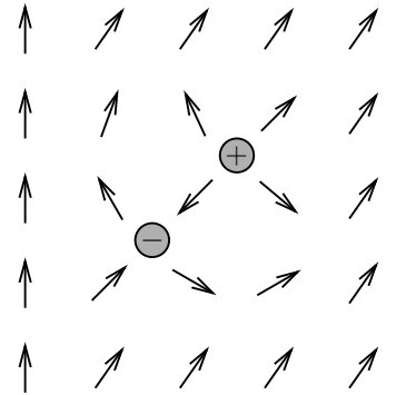
Fig. 34.12 A vortex dipole made from a vortex and antivortex in the same region of space. Notice that the fields may now be made uniform at infinity.
