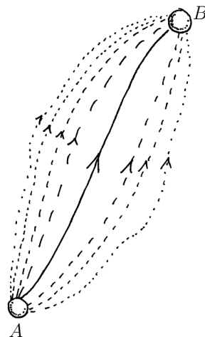
Fig. 23.3 The classical path is shown as a solid line, alternative paths allowed by quantum mechanics are shown as dashed lines.
