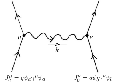
Fig. 39.1 The exchange of a virtual photon.
