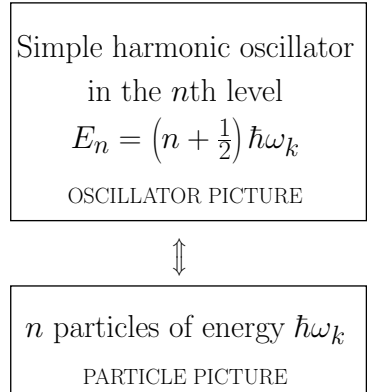
Fig. 2.6 The equivalence of the oscillator and particle pictures.
