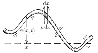
Fig. 1.5 Waves on a string. The displacement from equilibrium is \psi(x, t) and the equation of motion can be derived by considering an element of the string of length dx and mass \rho dx . The figure shows a short section in the middle of the string which is assumed to be tethered at either end so that \psi(0, t) = \psi(\ell, t) .
