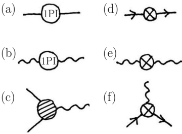
Fig. 41.1 Feynman diagrams for renormalized QED.
