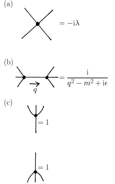
Fig. 19.10 Momentum space Feynman rules for \phi^4 theory.
