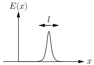
Fig. 29.8 The energy density of a kink is localized in an interval l .
