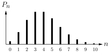
Fig. 27.1 The Poisson distribution P_n = e^{-|\alpha|^2} |\alpha|^{2n} / n! = e^{-\langle n \rangle} \langle n \rangle^n / n! plotted for |\alpha|^2 = \langle n \rangle = 4 . Note that a coherent state consists of a sum of harmonic oscillator states: the quantity P_n represents the probability of finding this coherent state in the n th harmonic oscillator state.
