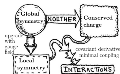
Fig. 38.4 The minimal coupling prescription in QED.
