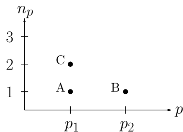
Fig. 3.2 A three-particle state given by |p_1p_2p_1\rangle can be written as |2100\dots\rangle in the occupation number representation.
