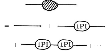
Fig. 33.3 Diagrammatic version of eqn 33.5.
