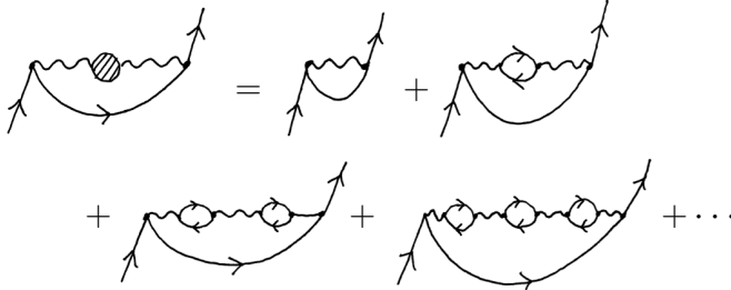
Fig. 43.17 The oyster diagram within the RPA.
