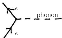
Fig. 44.1 The electron–phonon interaction vertex.
