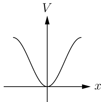
Fig. 50.1 A potential well.
