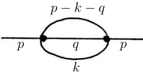
Fig. 32.3 The Saturn diagram.
