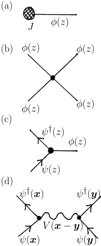
Fig. 19.2 Spacetime diagrams representing some commonly encountered interactions.
