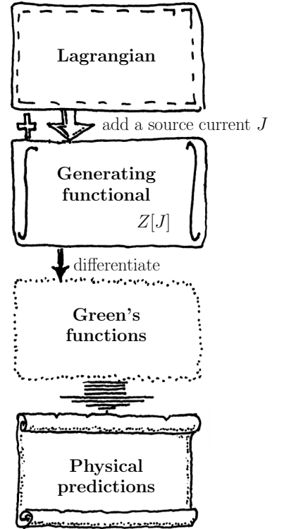
Fig. 22.1 Doing quantum field theory using generating functionals
