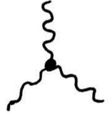
Fig. 46.2 The interaction of three W particles is possible in a gauge theory with local SU(2) symmetry.
