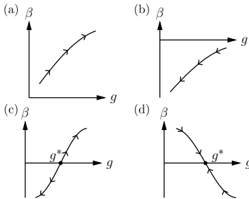
Fig. 34.2 Four examples of flows in a configuration space defined by a single coupling constant g , visualized by plotting \beta(g) = \frac{dg}{d \ln b} . Arrows show the direction that the length scale \ell \rightarrow \infty .
