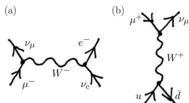
Fig. 47.5 Some example electroweak processes. (a) \mu^- + \nu_e \rightarrow \nu_\mu + e^- ; (b) positive pion decay involving quarks u and \bar{d} decaying into \mu^+ + \nu_\mu .
