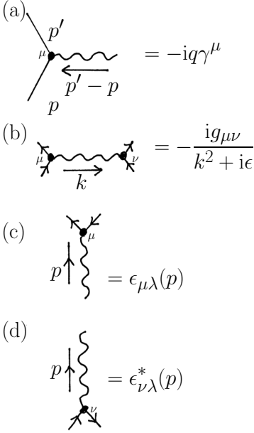
Fig. 39.2 The QED Feynman rules.
