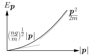
Fig. 42.2 The dispersion predicted by Bogoliubov's model. At low momentum the energy is linear in |\mathbf{p}| , at large momentum it is quadratic.
