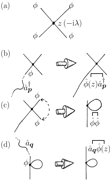
Fig. 19.3 Steps in drawing a diagram.
