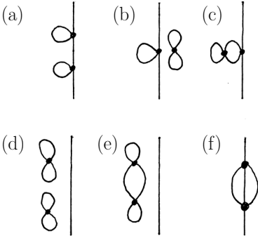
Fig. 19.8 All of the second-order \phi^4 diagrams.
