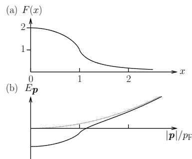
Fig. 43.4 (a) The function F(x) . (b) The energy of an electron in the Hartree-Fock approximation E_{\mathbf{p}} = \frac{p^2}{2m} + \Sigma_{\mathbf{p}}^{(F)} .
