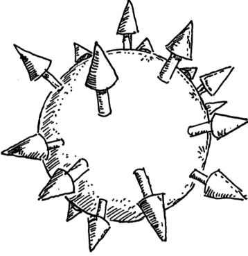
Fig. 49.4 The hedgehog solution.
