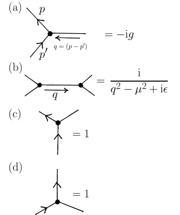
Fig. 20.5 Feynman rules for \psi^\dagger\psi\phi theory.
