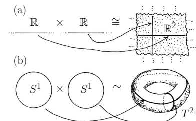
Fig. 29.2 A product space is constructed by attaching a copy of one space to every single point in another space. (a) A product space of the real line ( \mathbb{R} ) with itself produces the two-dimensional plane \mathbb{R}^2 . (b) The product of two circles ( S^1 ) produces the torus T^2 . A cup can be continuously deformed into a doughnut (a torus).
