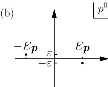
Fig. B.1 (a) Position of the pole in the complex E plane for \tilde{G}_0^+(E) . (b) Positions of the poles in the complex p_0 plane for the Feynman propagator for free scalar fields.
