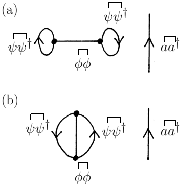
Fig. 20.3 Disconnected diagrams making second-order contributions.
