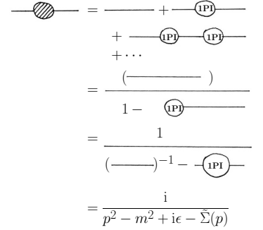
Fig. 33.4 Diagrammatic version of eqn 33.6
