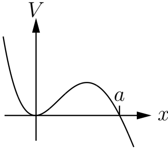
Fig. 50.8 A potential with a barrier.
