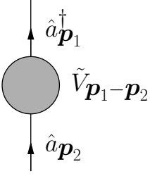
Fig. 4.5 A process represented by eqn 4.36. The sequence of events is: annihilate a particle with momentum \mathbf{p}_2 , count the potential energy \tilde{V}_{\mathbf{p}_1 - \mathbf{p}_2} , create a particle with momentum \mathbf{p}_1 .
