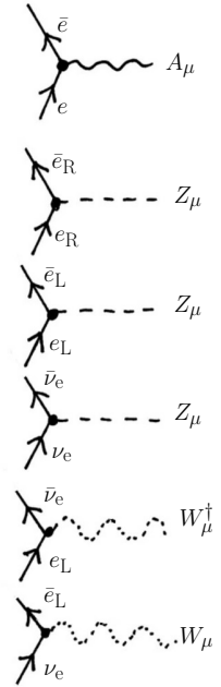
Fig. 47.4 The electroweak interaction vertices predicted by the Weinberg-Salam theory.
