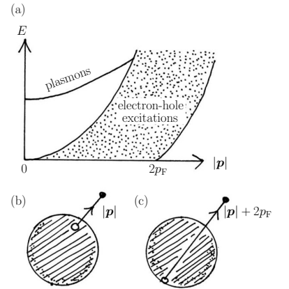
Fig. 43.18 (a) The excitation spectrum of a metal showing low-energy particle-hole quasiparticle excitations and the higher energy (collective) plasmon mode. A quasiparticle excitation with energy E_{\mathbf{p}} may be created with: (b) a momentum transfer |\mathbf{p}| , from one side of the Fermi surface, and (c) \approx |\mathbf{p}| + 2p_F from the other (and all momenta in between) leading to the continuum of states shown in the shaded region.
