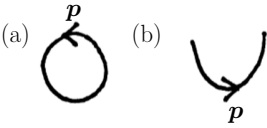
Fig. 43.6 Non-propagating lines.
