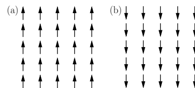
Fig. 26.2 For temperatures T < T_c the spins align along a single direction. The magnetization in (a) is different in (b), where each spin has been rotated by 180^\circ .
