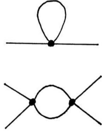
Fig. 35.2 One-loop Feynman diagrams in \phi^4 theory.
