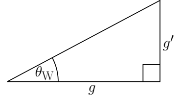
Fig. 47.3 Definition of the Weinberg angle \theta_W in terms of g' and g .
