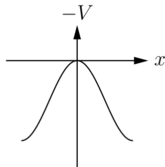
Fig. 50.2 An upside-down potential well, inverted by the Wick rotation to Euclidean space.
