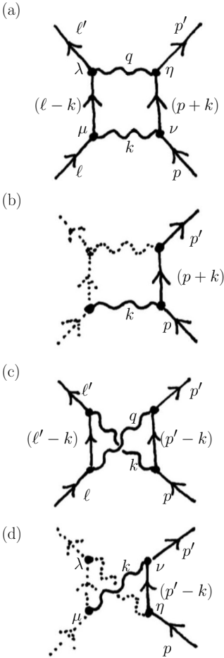
Fig. 39.8 Illustration of gauge invariance in the diagrammatic language used in Exercise 39.4.
