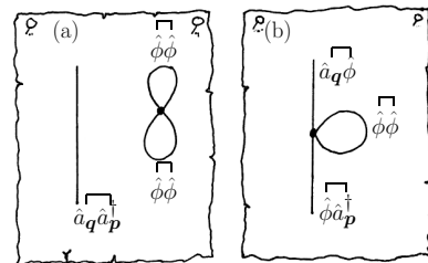
Fig. 19.4 First-order contributions in \hat{\phi}^4 theory. (a) A disconnected diagram with two connected parts. (b) Connected diagram with one loop.
