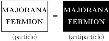
Fig. 48.1 A Majorana fermion is its own antiparticle.
