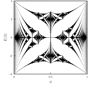
Fig. 45.1 The Hofstadter butterfly.
