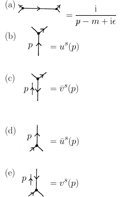
Fig. 38.2 Feynman rules for fermions.
