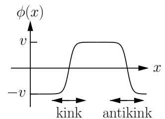
Fig. 29.9 A kink and antikink.
