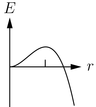
Fig. 50.13 The energy of a bubble of gas of radius r in a superheated liquid.
