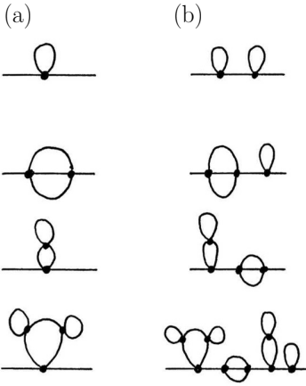
Fig. 33.1 (a) Some 1PI diagrams from \phi^4 theory. They can't be turned into two meaningful diagrams by cutting one propagator line. (b) Diagrams that aren't 1PI. All can be turned into legitimate 1PI diagrams by cutting at some point along the horizontal line.
