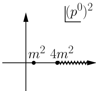
Fig. B.5 The pole structure of the full propagator in eqn. B.24.
