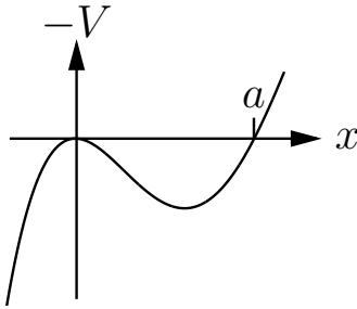
Fig. 50.9 The barrier potential turned upside-down.
