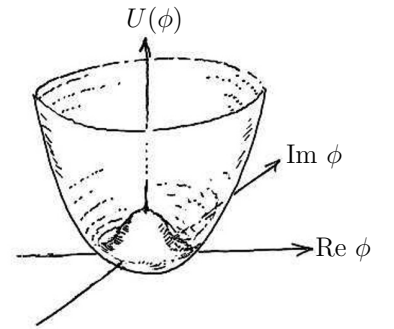
Fig. 47.1 The potential of the Higgs field.
