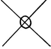
Fig. 32.2 The C -counterterm.
