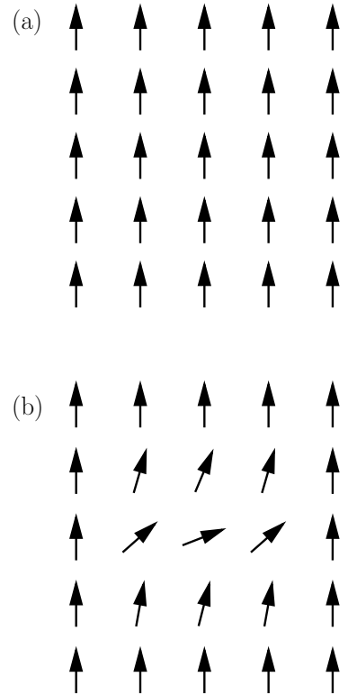
Fig. 42.3 (a) Order in the superfluid corresponds to a uniform phase angle across the entire system. This is represented on a lattice here. (b) A gradient in the phase \nabla \theta(x) results in a current in the superfluid.
