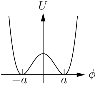
Fig. 29.5 The double well potential.
