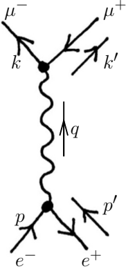
Fig. 39.3 A first QED process: e^+e^- \rightarrow \mu^+\mu^- .
