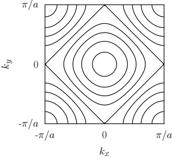
Fig. 4.7 The tight-binding model for a two-dimensional square lattice. Contours showing lines of constant energy E_{\mathbf{k}} based on eqn 4.50 are plotted as a function of k_x and k_y . For t > 0 , the lowest E_{\mathbf{k}} occurs at (k_x, k_y) = (0, 0) , the centre of this plot. For t < 0 , the lowest E_{\mathbf{k}} occurs at the corners, (k_x, k_y) = (\pm \frac{\pi}{a}, \pm \frac{\pi}{a}) .
