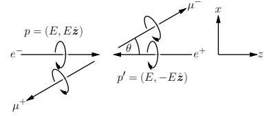
Fig. 39.4 Kinematics for our first QED process.
