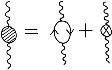
Fig. 41.4 The lowest order correction to the photon propagator and the counterterm that prevents its divergence.
