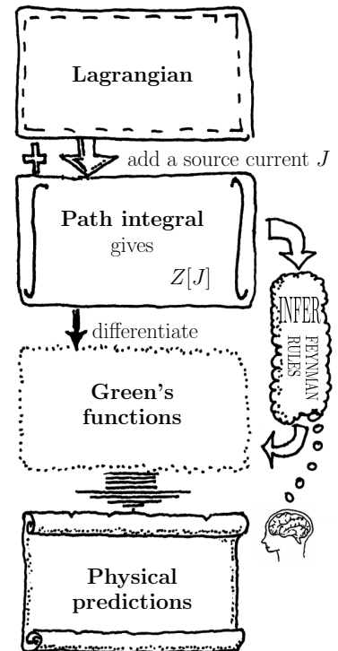
Fig. 24.1 Using functional integrals to do quantum field theory.
