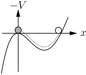
Fig. 50.9 The barrier potential turned upside-down.
