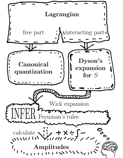
Fig. 19.7 The process of deriving the Feynman rules.
