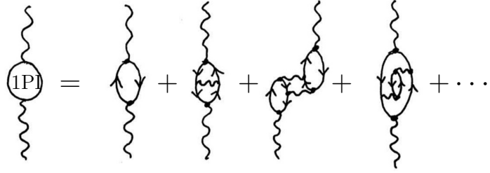
Fig. 43.13 Some of the diagrams contributing to i\tilde{\Pi}(q) .
