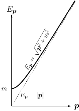
Fig. 7.2 The dispersion relation E_p = \sqrt{p^2 + m^2} for a massive particle.
