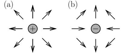
Fig. 34.10 (a) A vortex. (b) An antivortex.
