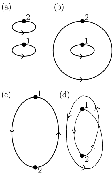
Fig. 30.1 Examples of ways of exchanging particles. (a) and (b) are type A processes, where the particles end up at the same positions. In case (b) one particle loops around the other once in the exchanging process. (c) and (d) are type B processes where the particles exchange positions. In case (d) one particle loops once around the other during the exchange.
