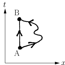
Fig. 5.2 The straight-line path from A to B has a larger \int_a^b ds than the wiggly one (because c dt > \sqrt{c^2 dt^2 - dx^2} ), even though the wiggly one looks longer.
