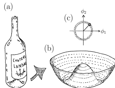
Fig. 26.6 (a) The potential for the SO(2) symmetry breaking looks like the bottom of a punted wine bottle. (b) There is a maximum at the point \phi_1 = \phi_2 = 0 , but surrounding this there is a set of minima which lie on a circle. (c) The circle of minima are shown on a \phi_1 - \phi_2 plot (this is therefore viewing the surface sketched in (b) from 'above'). The symmetry can then be broken by choosing a particular point in the circle of minima and setting this to be the ground state. We can then examine small deviations away from that point.
