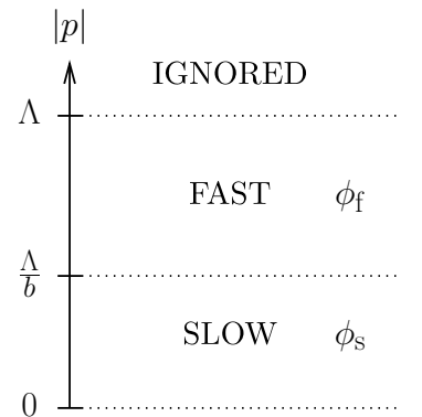
Fig. 34.5 Components in momentum space are divided up into slowly varying and fast varying, with any component with |p| > \Lambda being ignored.
