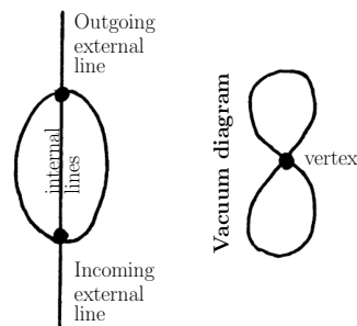
Fig. 19.5 The anatomy of a disconnected third-order diagram.
