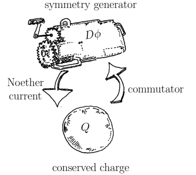
Fig. 10.3 Noether's theorem for the field \phi .
