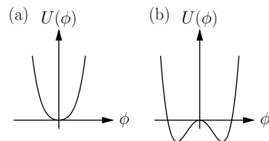
Fig. 26.5 Equation 26.5 for (a) \mu^2 > 0 with a minimum at \phi = 0 and (b) for \mu^2 < 0 with minima at \pm\sqrt{6\mu^2/\lambda} .
