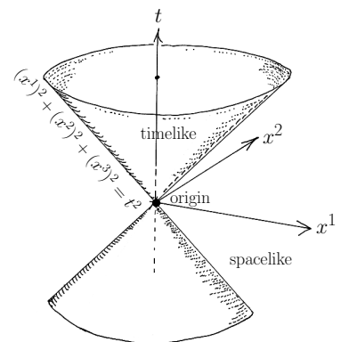
Fig. 8.2 A particle shouldn’t be observed outside its forward light-cone. If it starts at the origin, it should only be able to make time-like journeys.
