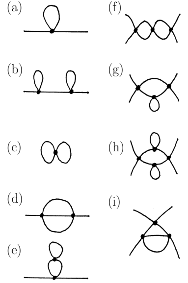
Fig. 19.6 Examples of diagrams in \phi^4 theory.
