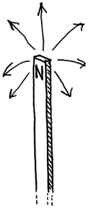
Fig. 49.2 You can think of a monopole as originating from an extremely long bar magnet.
