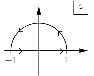
Fig. B.2 An example of a contour in the complex z plane.
