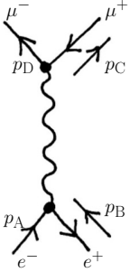
Fig. 40.5 The s -channel process e^-e^+ \rightarrow \mu^-\mu^+ .
