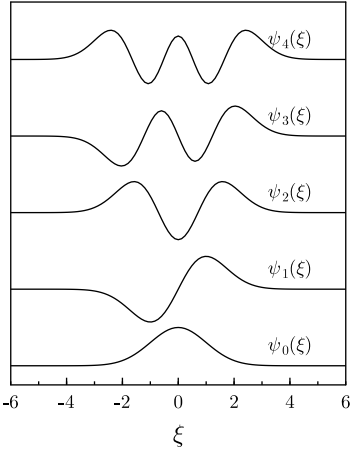
Fig. 2.2 Eigenfunctions of the simple harmonic oscillator.
