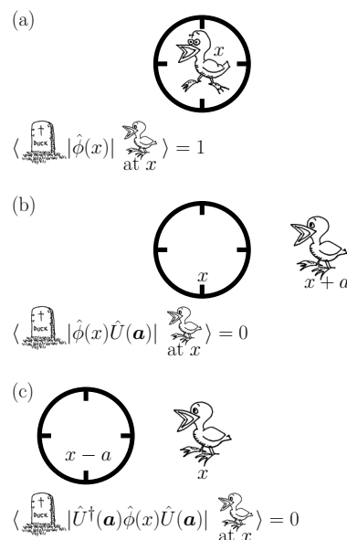
Fig. 9.3 The field operator \hat{\phi}(\mathbf{x}) acting on a localized state is pictured as a sniper's bullet shooting a duck located at position \mathbf{x} . (a) Dead on target, the state of a dead duck has perfect overlap with the state produced by acting \hat{\phi}(\mathbf{x}) on the live duck at \mathbf{x} . (b) Translating the state results in a miss, as does (c) translating the operator.
