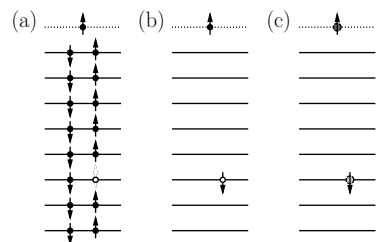
Fig. 31.3 (a) The non-interacting electron gas with a single electron above the Fermi level. (b) The particle excitations in the non-interacting electron gas. (c) The quasiparticles in the interacting electron gas [identical to (b) but with renormalized masses].
