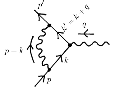
Fig. 41.10 The third-order diagram which contributes to F_2(0) .
