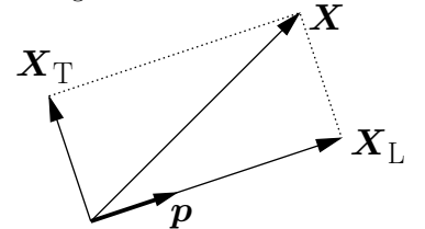
Fig. 13.2 Projecting a three-vector \mathbf{X} along the direction of a vector \mathbf{p} .
