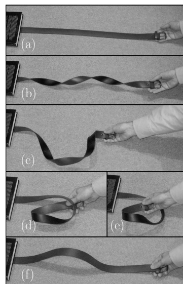
Fig. 15.7 Dirac’s scissor trick is more easily demonstrated with a belt with one end free and the other end held fixed by placing it under a book. [Figure from S. J. Blundell, Magnetism: A Very Short Introduction , OUP (2012).]
