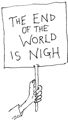
Fig. 50.17 We have essentially no warning of the coming of the true vacuum. However, we can give some advance notice of the imminent end of this book.
