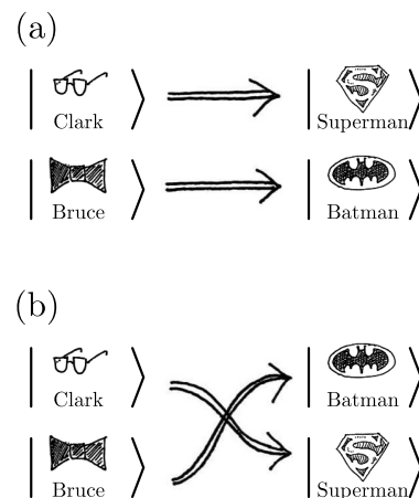
Fig. 31.6 Turning on interactions changes the states but the energy levels shouldn't cross during the turning on process. Thus we can have (a) but not (b).
