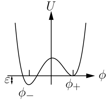
Fig. 50.12 False vacuum potential.
