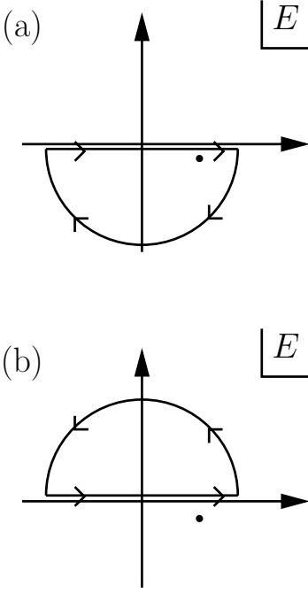
Fig. B.3 (a) The contour completed in the lower half-plane enclosing the pole. Note that the direction here is clockwise, earning us an extra minus sign. (b) The contour completed in the upper half-plane. No poles are enclosed so the answer is given by Cauchy's theorem.
