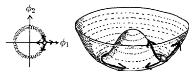
Fig. 26.7 Breaking symmetry at the position (\phi_1, \phi_2) = \left(+\sqrt{\frac{6\mu^2}{\lambda}}, 0\right) . There are two possible excitations: the particle can oscillate up and down in the \phi_1 direction (a massive excitation) or trundle round in the gutter (a massless excitation).
