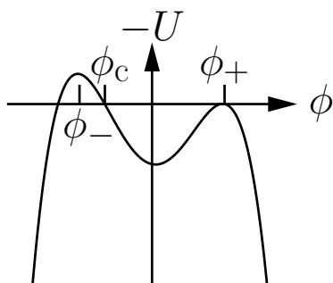
Fig. 50.14 False vacuum potential in Euclidean space.
