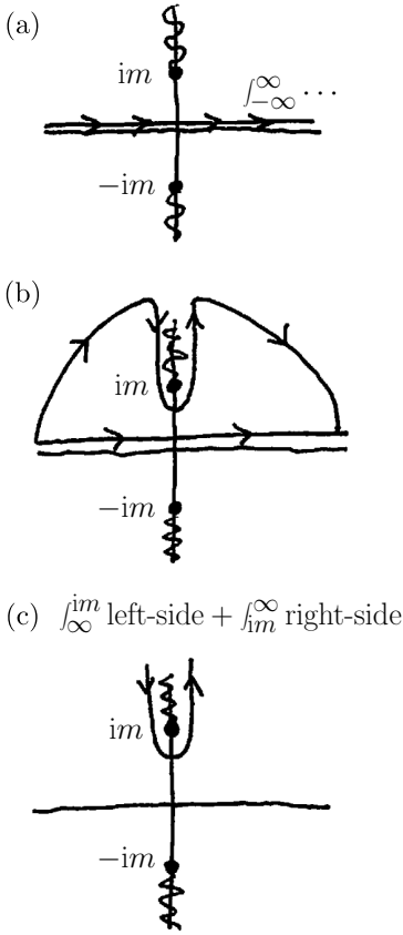
Fig. 8.3 The contour integration.
