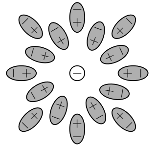
Fig. 41.6 Screening in QED.
