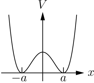
Fig. 50.3 The double potential well.
